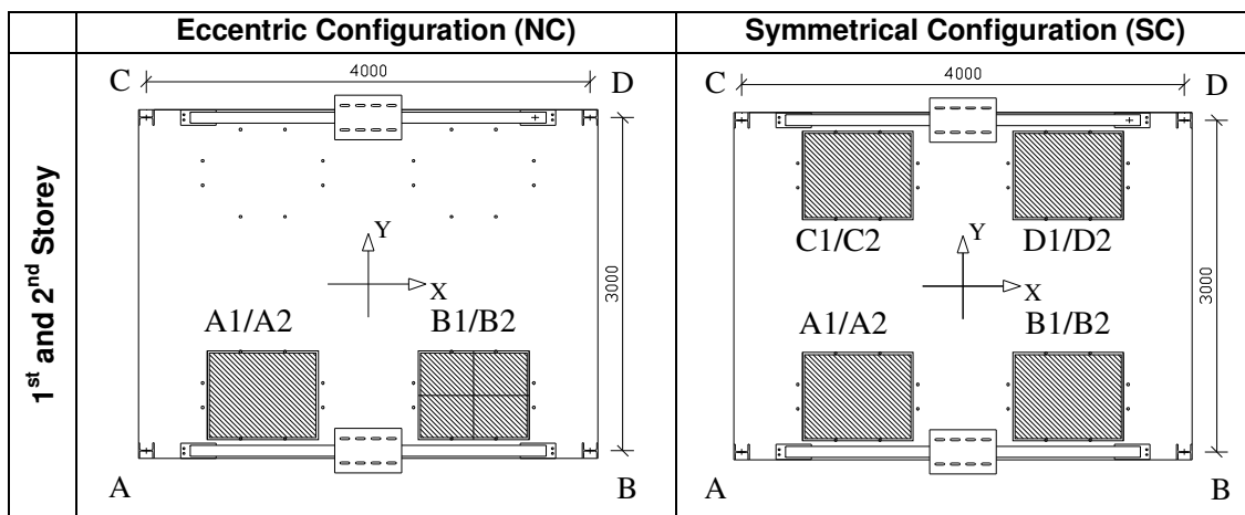
Figure 2. Concrete block positions for symmetrical (SC) and eccentric (NC) mass configurations
