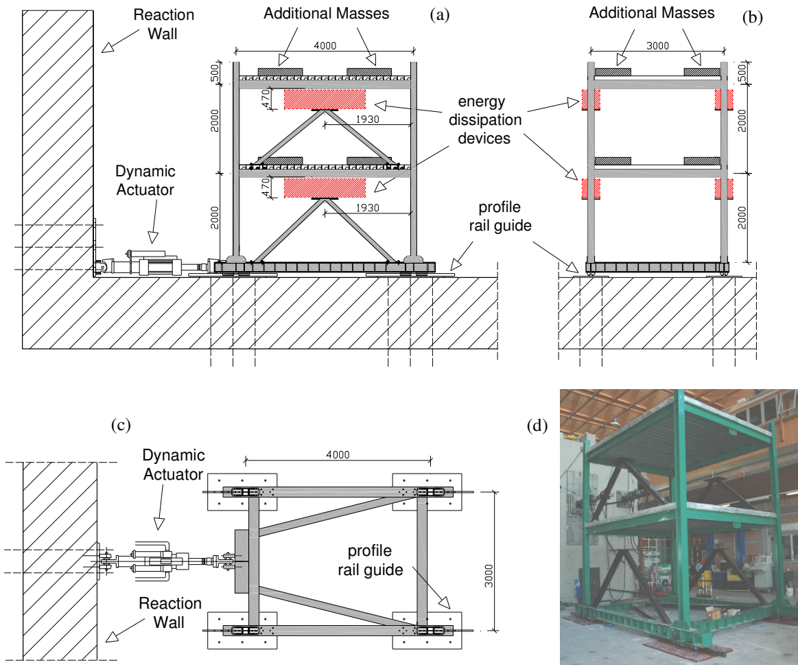
Figure 1. Structural model selected for the tests (a) Frame (Test) X Direction; (b) Frame Y Direction; (c) Shaking table plan; (d) 3-D view of the test rig
