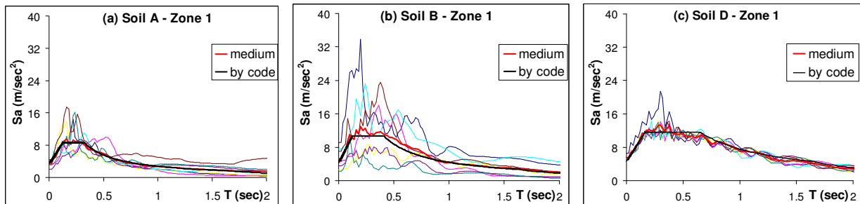
Figure 4. Elastic response spectra of sets of natural accelerograms for Seismic Zone 1 and (a) soil type A; (b) soil type B and (c) soil type D; time scaled by t/\sqrt{1.5} .
