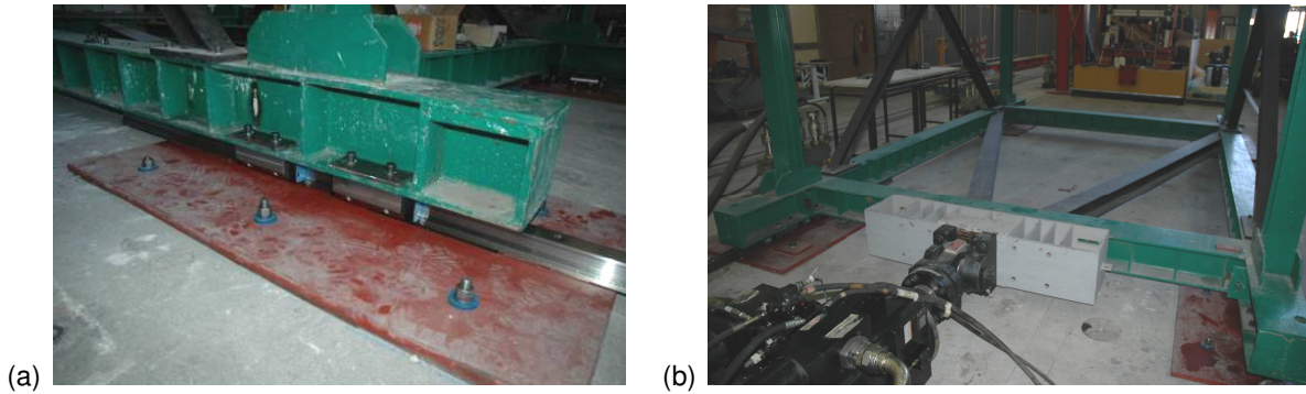
Figure 3. Shaking table: (a) SKF profile rail guide; (b) Model base
