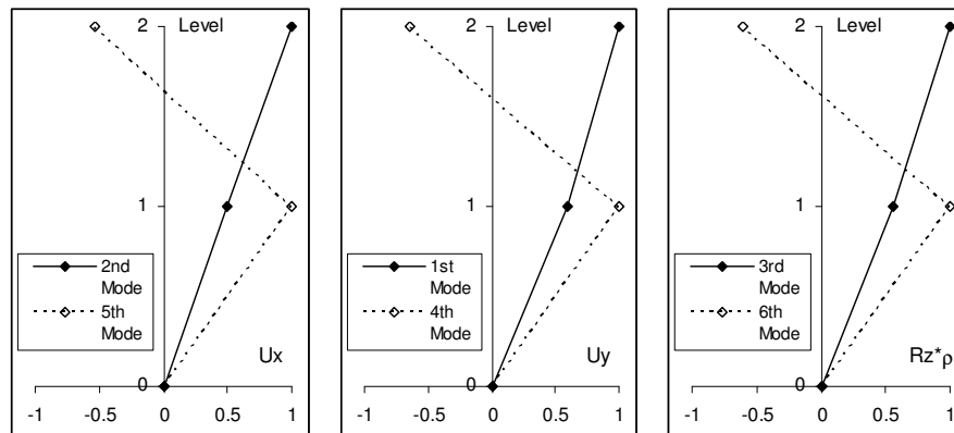
Figure 5. Model mode shapes of the SB configuration for the test direction
